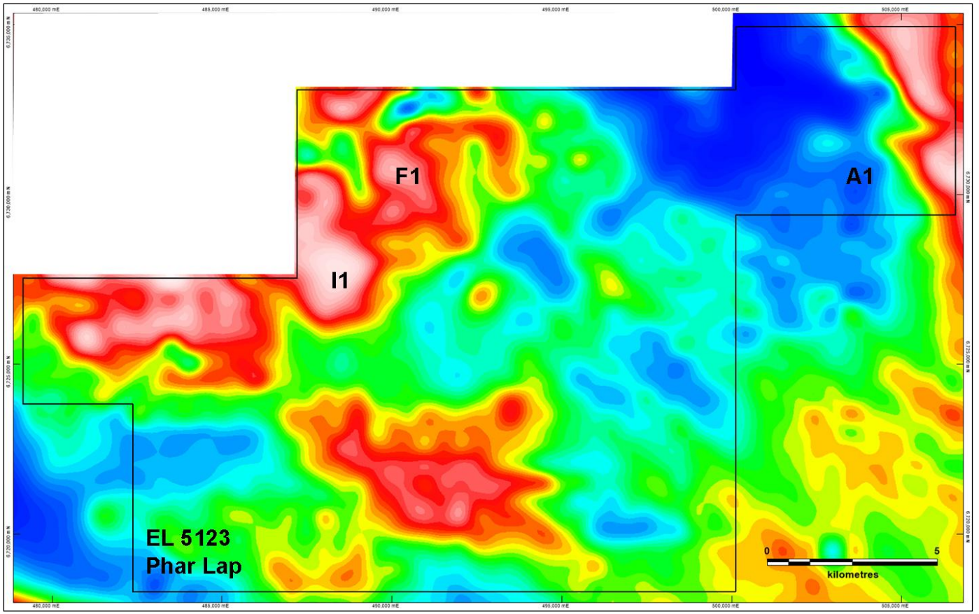
Figure 2. Newly acquired gravity data merged with existing gravity data highlighting the three potential ICG targets (I1, F1 & A1).
